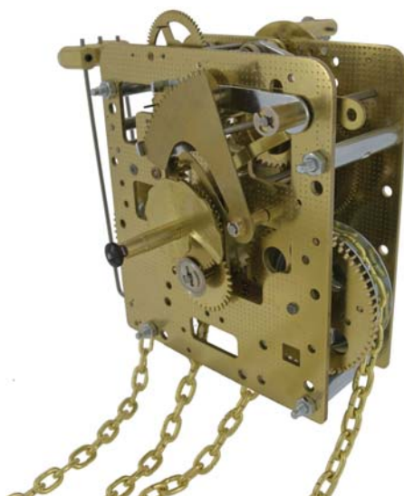
Hermle 241.030 8 day bim bam gong, weight driven clock movement
