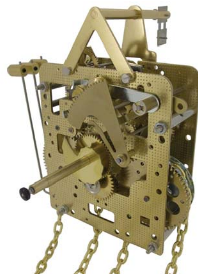
Hermle 241.033H 8 day bim bam gong, weight driven clock movement, 48.5mm shaft
