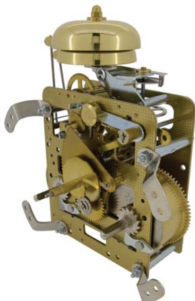
Hermle 150.080 8 day bim bam bell, key wound clock movement
