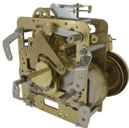
Hermle 150.070 8 day bim bam bell, key wound clock movement
