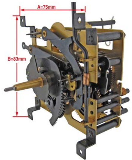
Regula 25 - 1 Day Cuckoo Clock Movement
