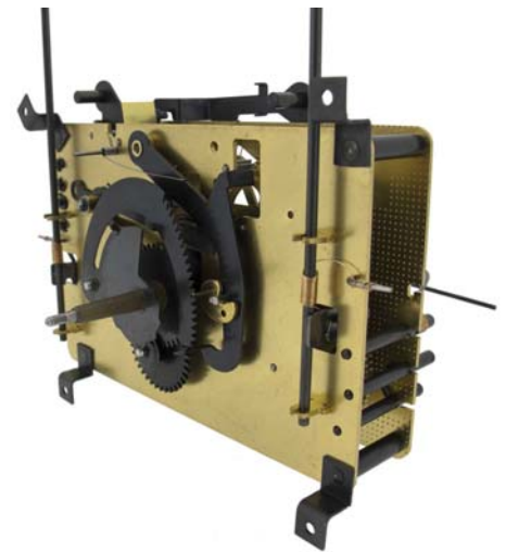
Regula 71 - 1 Day Cuckoo Clock Movement - Cuckoo & Quail
